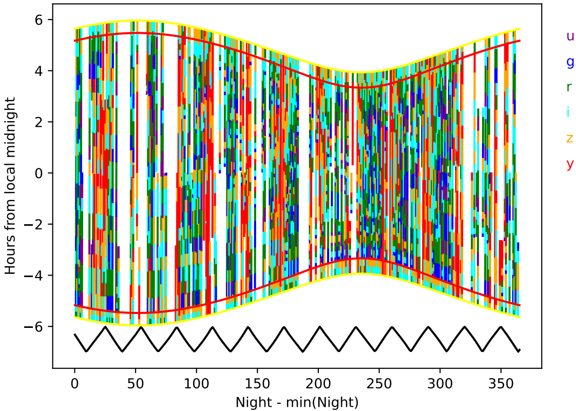
ddf_acor_sf15_lsf30_lsr10_v3.4_10yrs year 7-8: Hourglass
