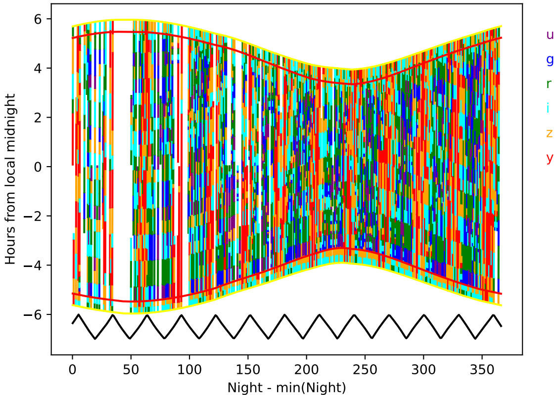
ddf_acor_sf15_lsf30_lsr10_v3.4_10yrs year 6-7: Hourglass
