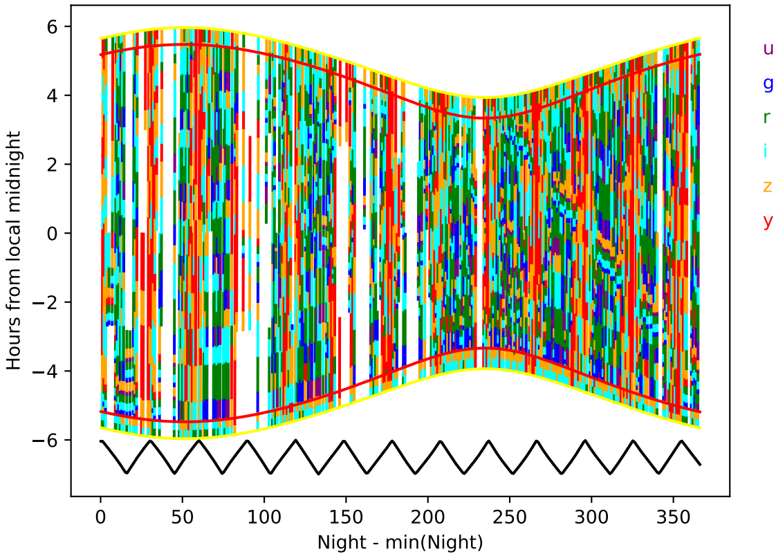
ddf_acor_sf15_lsf30_lsr10_v3.4_10yrs year 1-2: Hourglass
