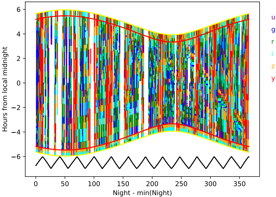
ddf_acor_sf15_ls30_lsr10_v3.4_10yrs year 0-1: Hourglass
