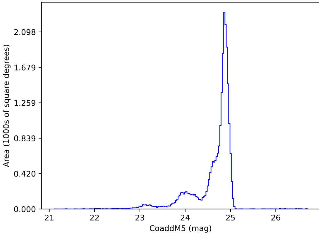
ddf_acor_sf15_lsf30_lsr10_v3.4_10yrs y: CoaddM5
