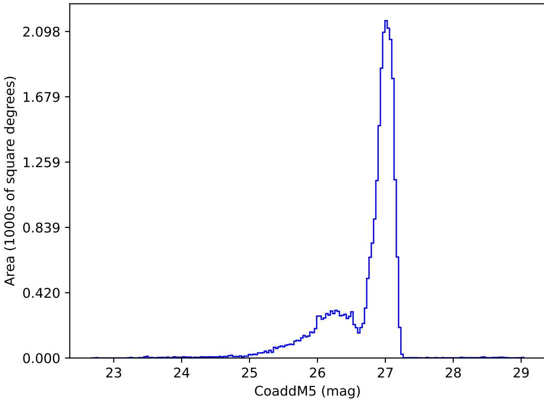
ddf_acor_sf15_lsf30_lsr10_v3.4_10yrs r: CoaddM5
