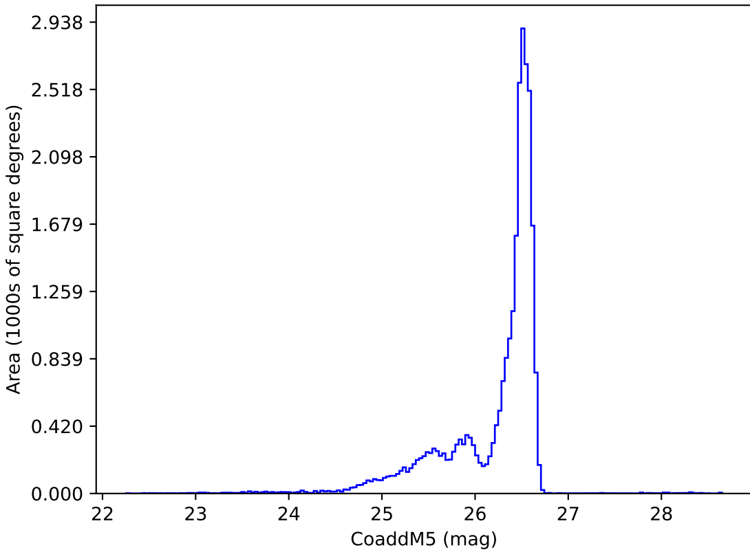
ddf_acor_sf15_lsf30_lsr10_v3.4_10yrs i: CoaddM5
