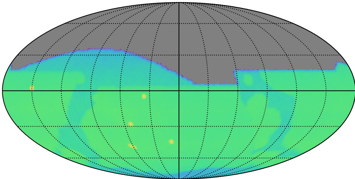
ddf_acor_sf15_lsf30_lsr10_v3.4_10yrs : CoaddM5
