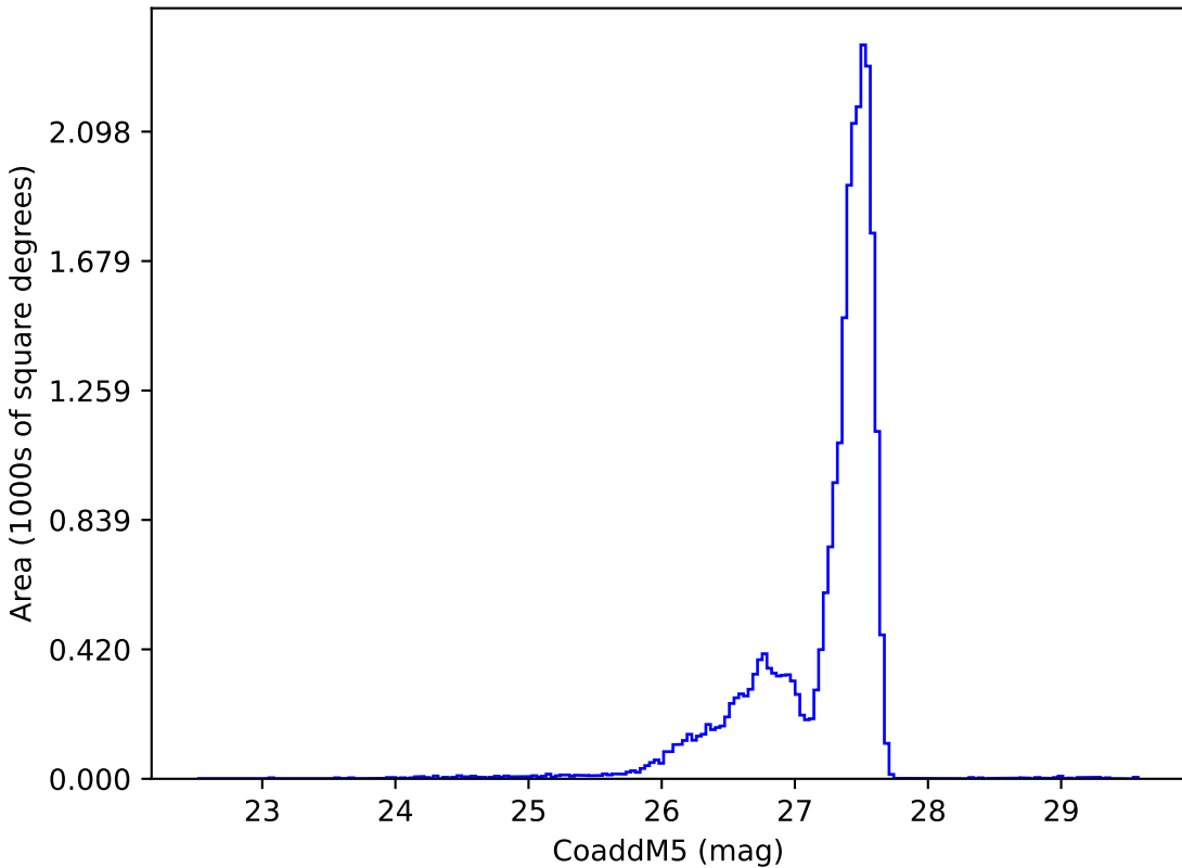
ddf_acor_sf15_lsf30_lsr10_v3.4_10yrs : CoaddM5
