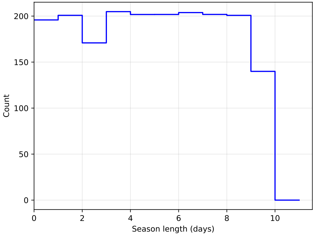
ddf_acor_sf15_lsf30_lsr10_v3.4_10yrs DD:ECDFS all bands: SeasonLength
