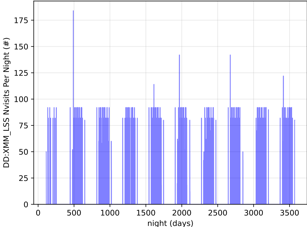
ddf_acor_sf15_lsf30_lsr10_v3.4_10yrs all bands: DD:XMM_LSS Nvisits Per Night
