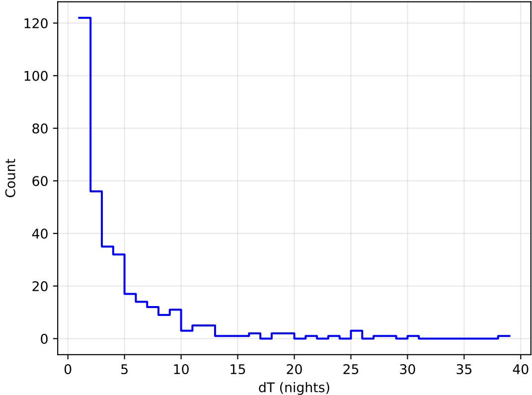
ddf_acor_sf15_lsf30_lsr10_v3.4_10yrs all bands: DD:WFD Delta Nights Histogram
