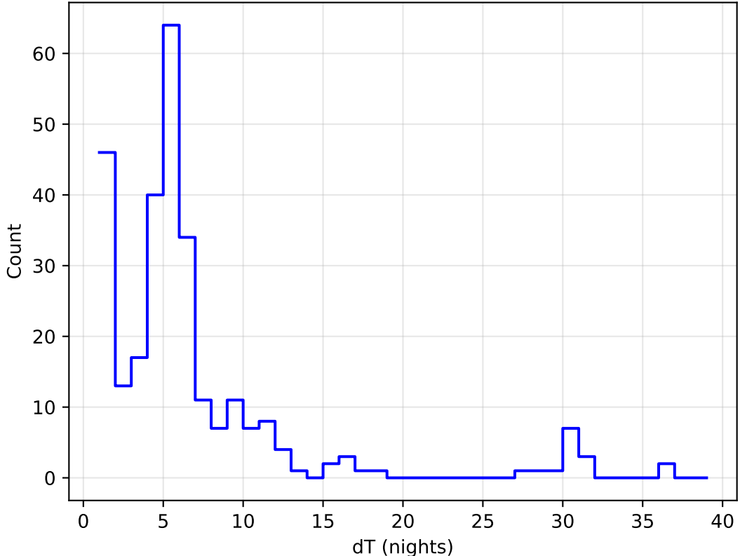
ddf_acor_sf15_lsf30_lsr10_v3.4_10yrs all bands: DD:ELAISS1 Delta Nights Histogram
