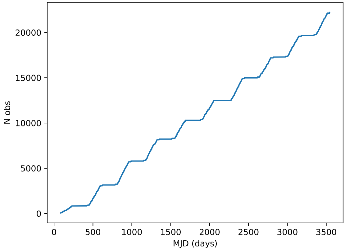
ddf_acor_sf15_lsf30_lsr10_v3.4_10yrs all bands: DD:ELAISS1 Cumulative NVisits
