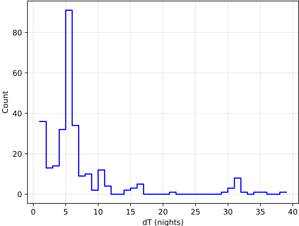
ddf_acor_sf15_lsf30_lsr10_v3.4_10yrs all bands: DD:EDFS Delta Nights Histogram
