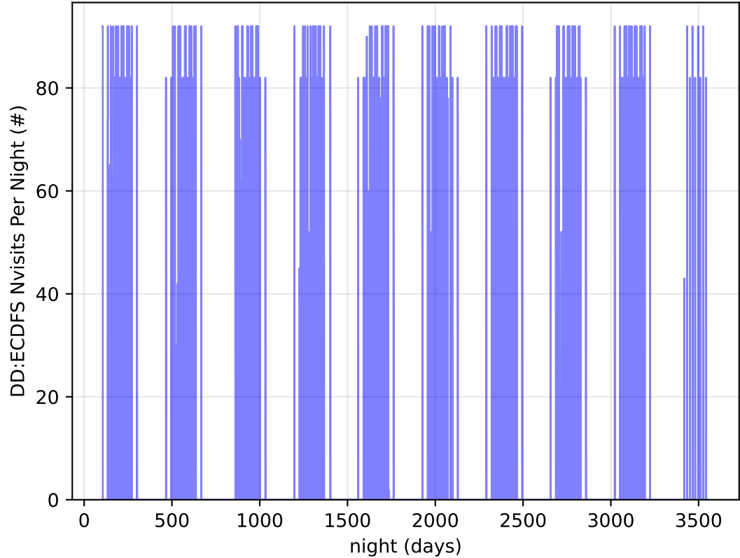
ddf_acor_sf15_lsf30_lsr10_v3.4_10yrs all bands: DD:ECDFS Nvisits Per Night
