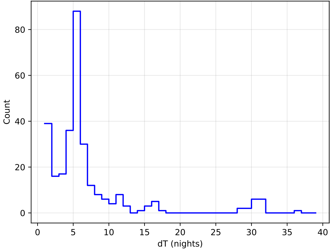
ddf_acor_sf15_lsf30_lsr10_v3.4_10yrs all bands: DD:ECDFS Delta Nights Histogram
