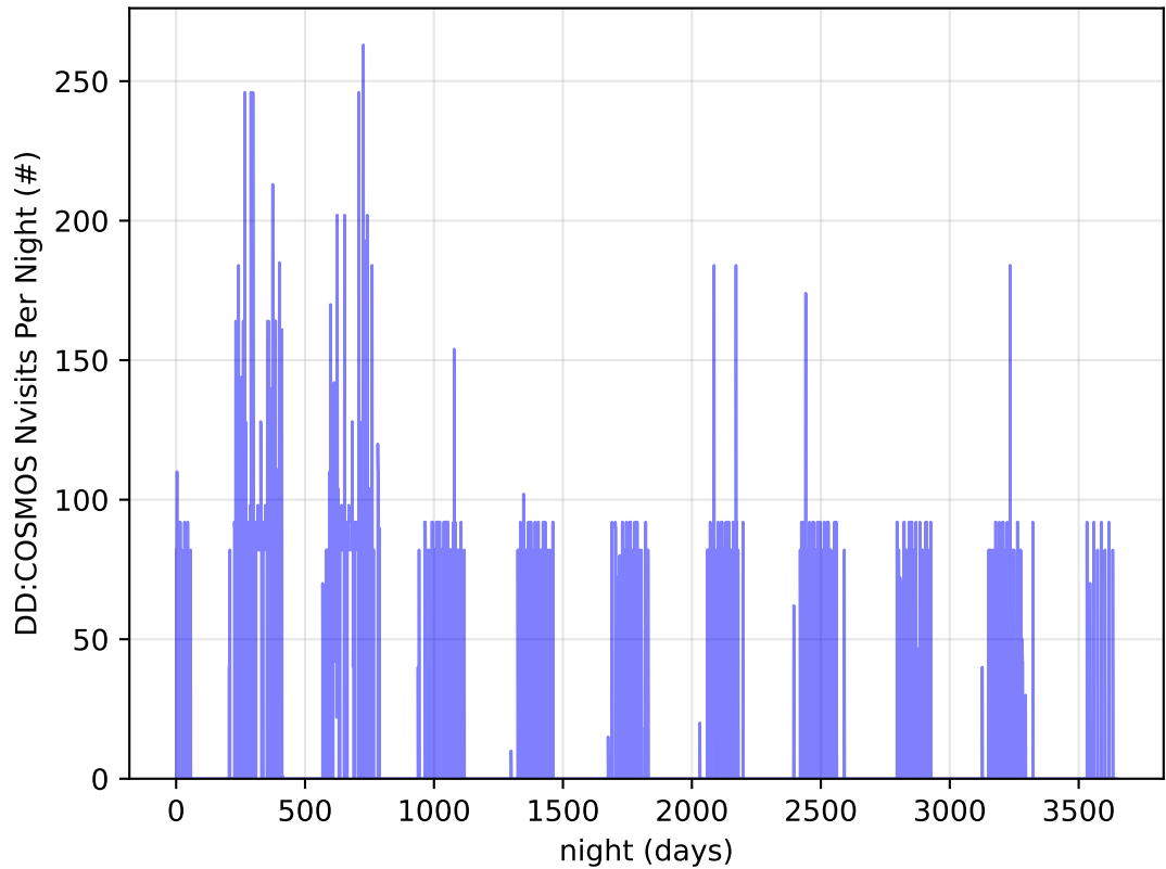
ddf_acor_sf15_lsf30_lsr10_v3.4_10yrs all bands: DD: COSMOS Nvisits Per Night
