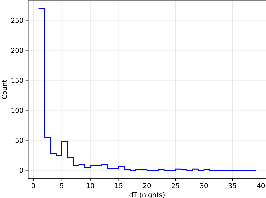
ddf_acor_sf15_Isf30_Isr10_v3.4_10yrs all bands: DD:COSMOS Delta Nights Histogram
