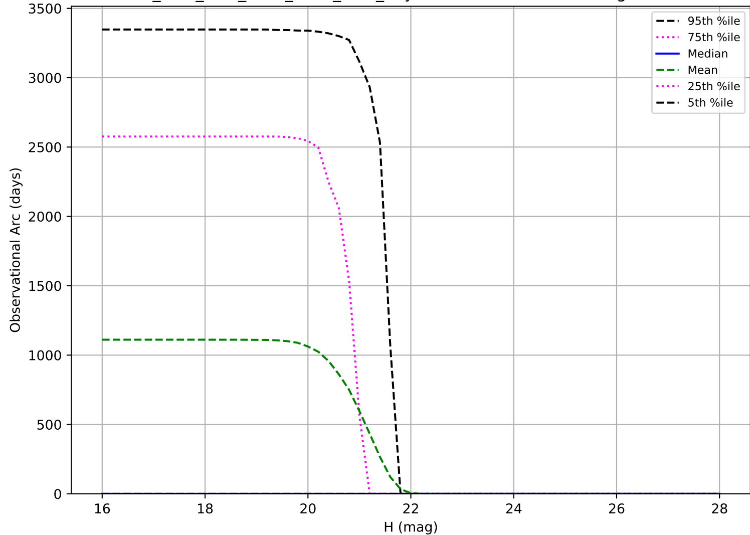
ddf_acor_sf15_lsf20_lsr50_v3.4_10yrs: Observational Arc Length Vatira
