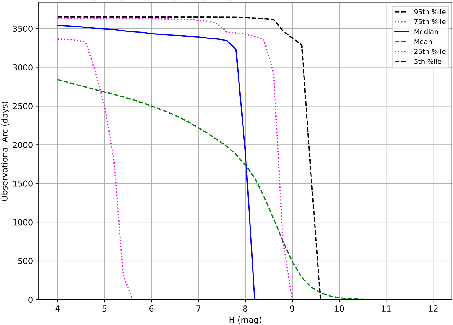
ddf_acor_sf15_Isf20_Isr50_v3.4_10yrs: Observational Arc Length TNO
