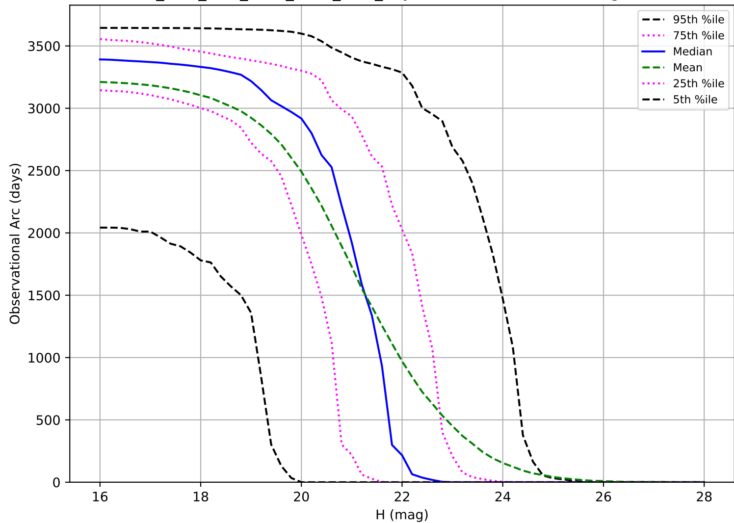
ddf_acor_sf15_lsf20_lsr50_v3.4_10yrs: Observational Arc Length PHA
