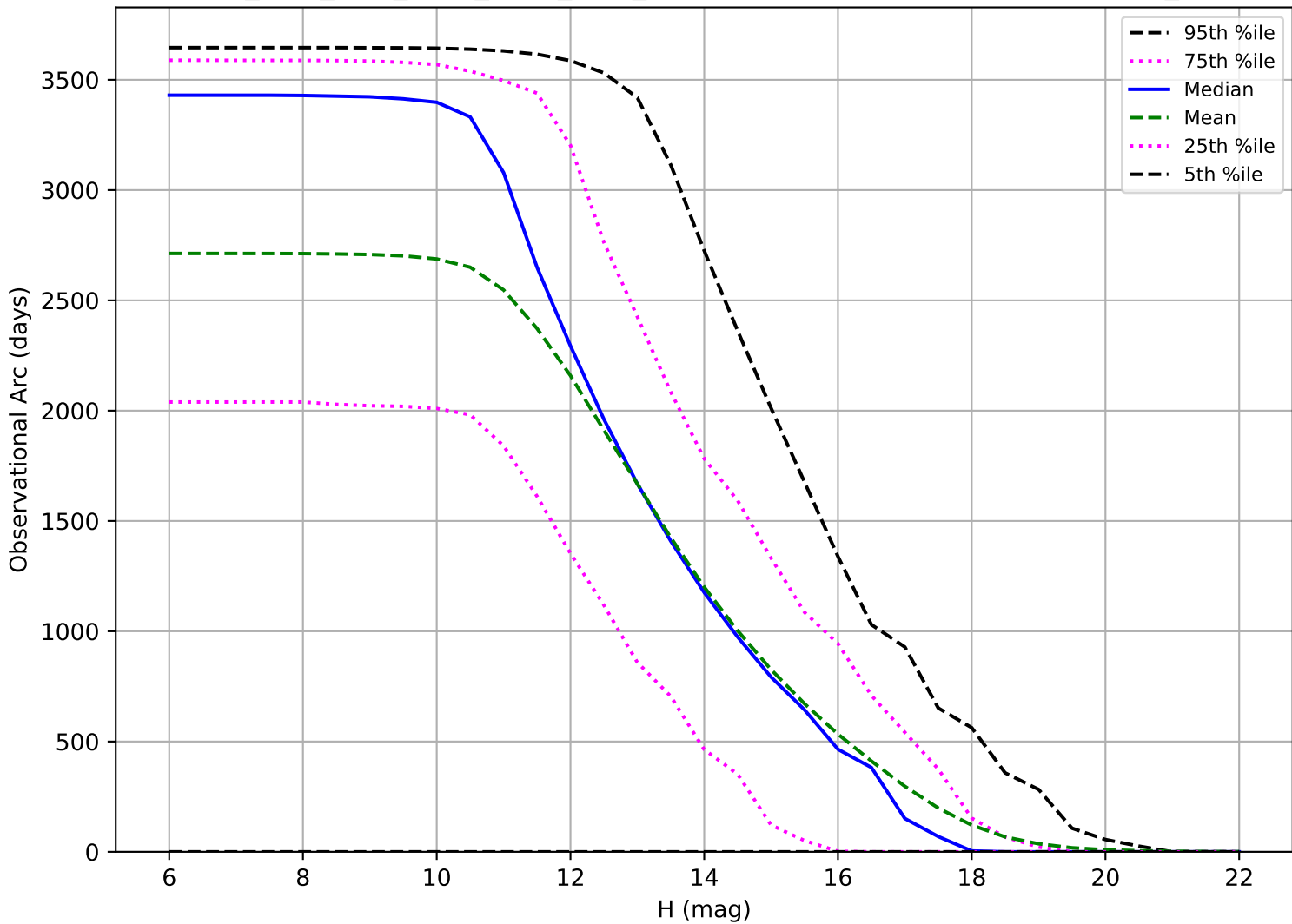
ddf_acor_sf15_lsf20_lsr50_v3.4_10yrs: Observational Arc Length OCC_r5
