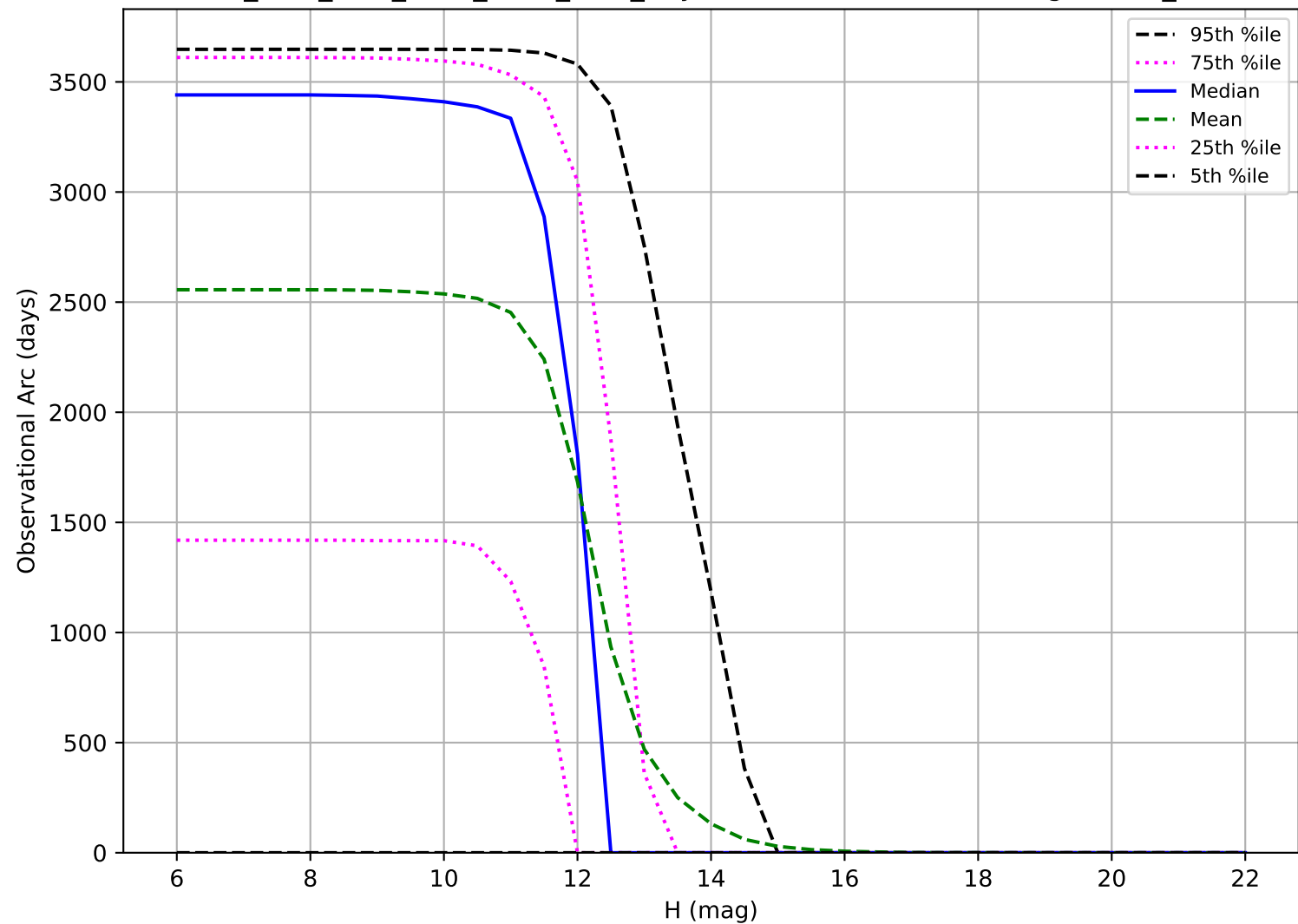
ddf_acor_sf15_lsf20_lsr50_v3.4_10yrs: Observational Arc Length OCC_r20
