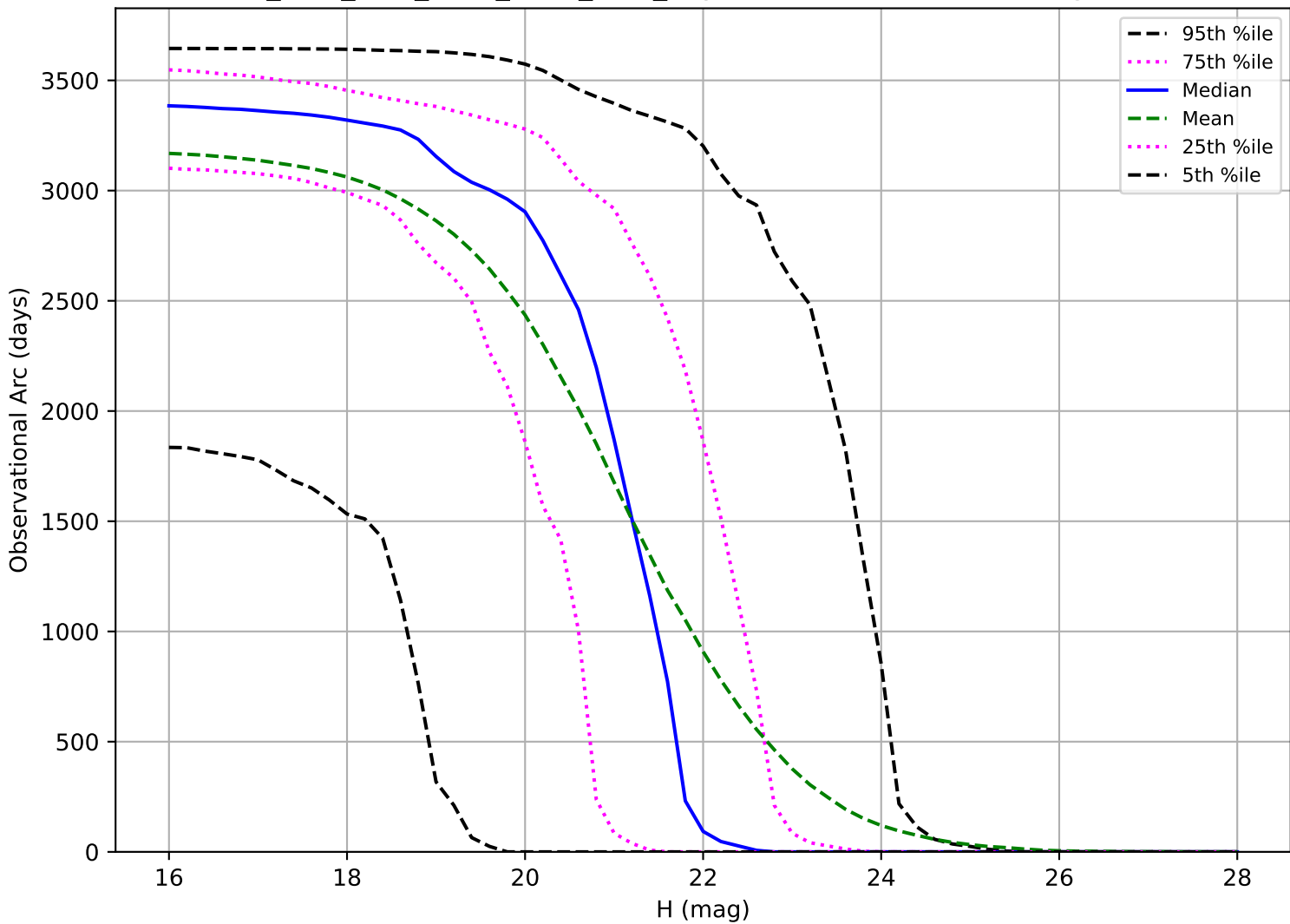
ddf_acor_sf15_lsf20_lsr50_v3.4_10yrs: Observational Arc Length NEO
