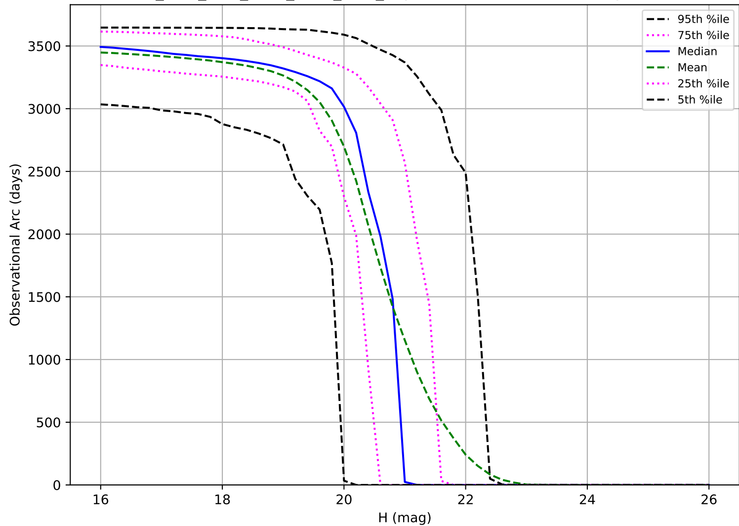
ddf_acor_sf15_lsf20_lsr50_v3.4_10yrs: Observational Arc Length MBA
