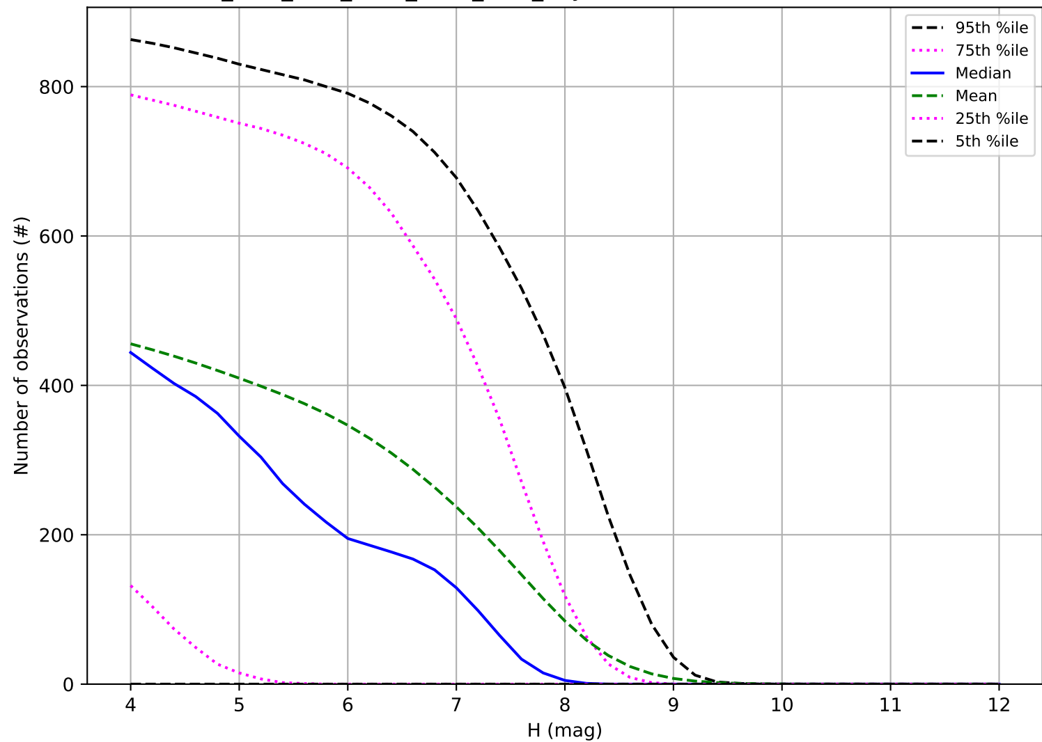
ddf_acor_sf15_lsf20_lsr50_v3.4_10yrs: Number of observations TNO
