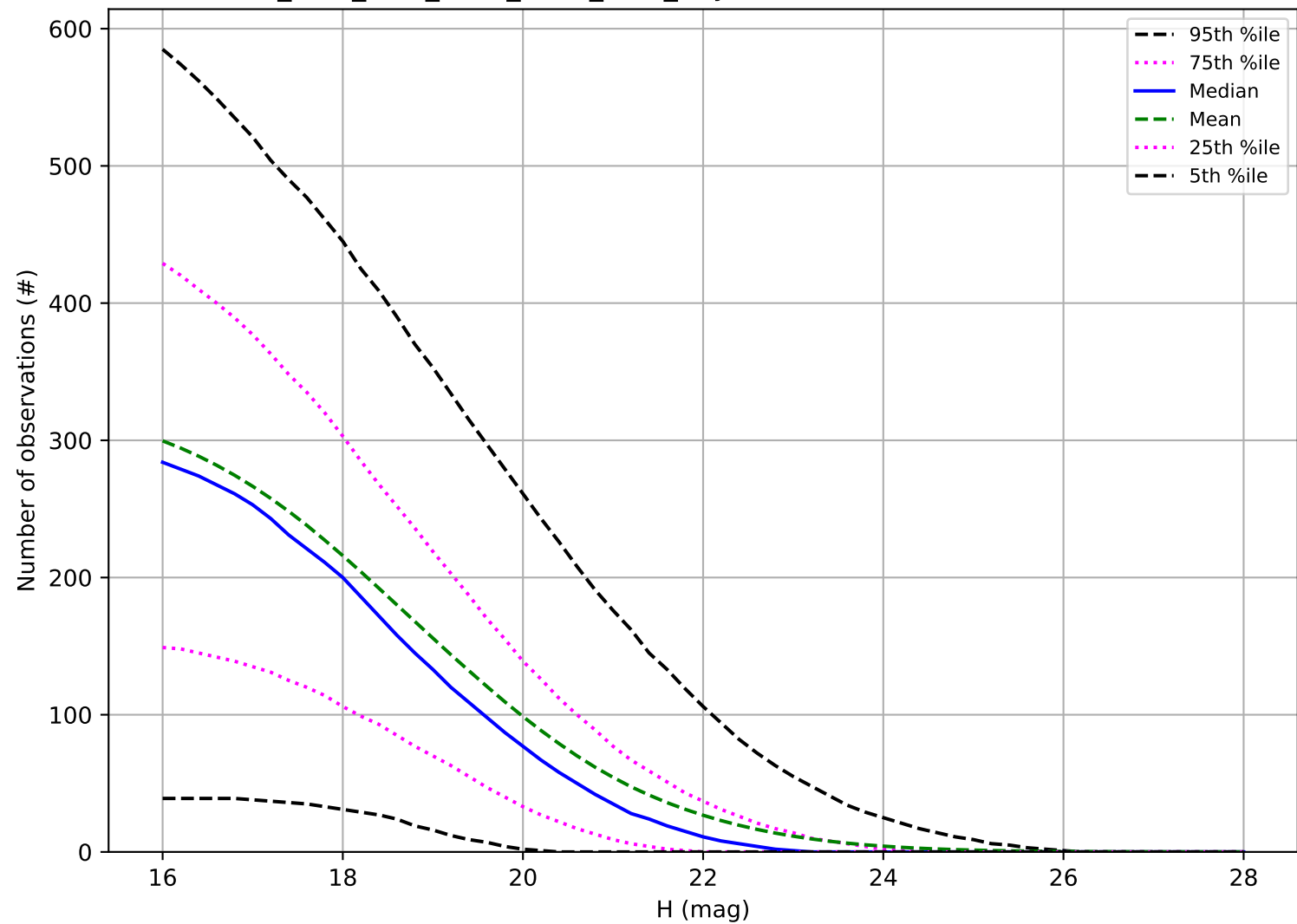
ddf_acor_sf15_lsf20_lsr50_v3.4_10yrs: Number of observations PHA
