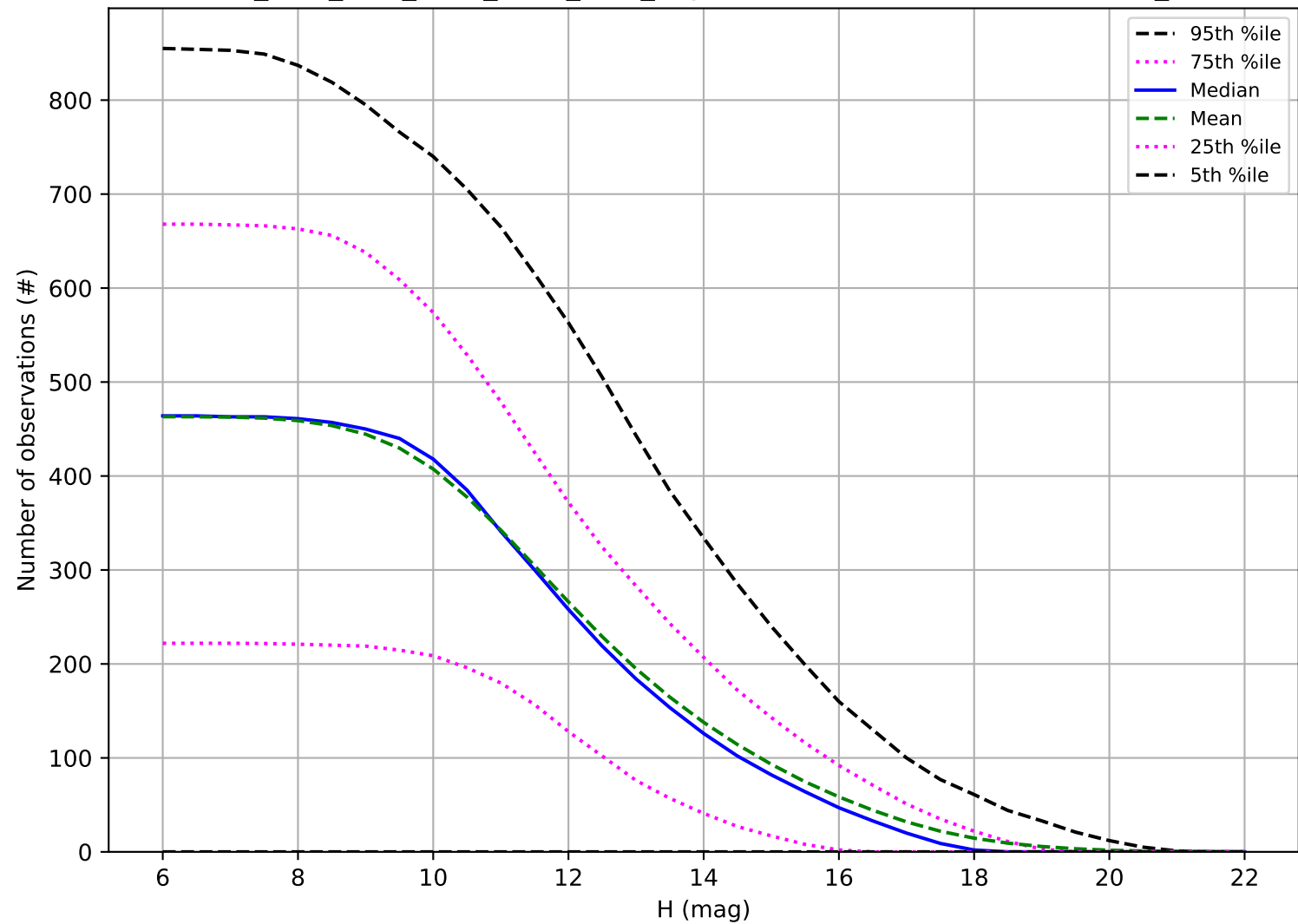
ddf_acor_sf15_lsf20_lsr50_v3.4_10yrs: Number of observations OCC_r5
