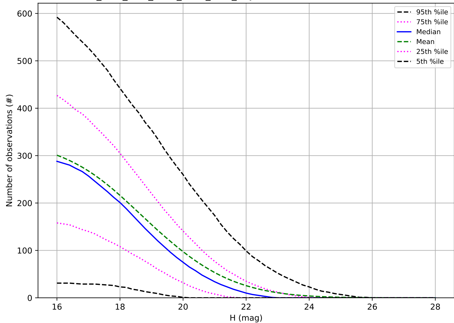
ddf_acor_sf15_lsf20_lsr50_v3.4_10yrs: Number of observations NEO
