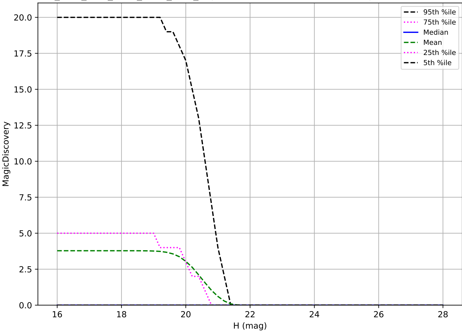
ddf_acor_sf15_lsf20_lsr50_v3.4_10yrs: Vatra 6 detections in 60 nights detection loss
