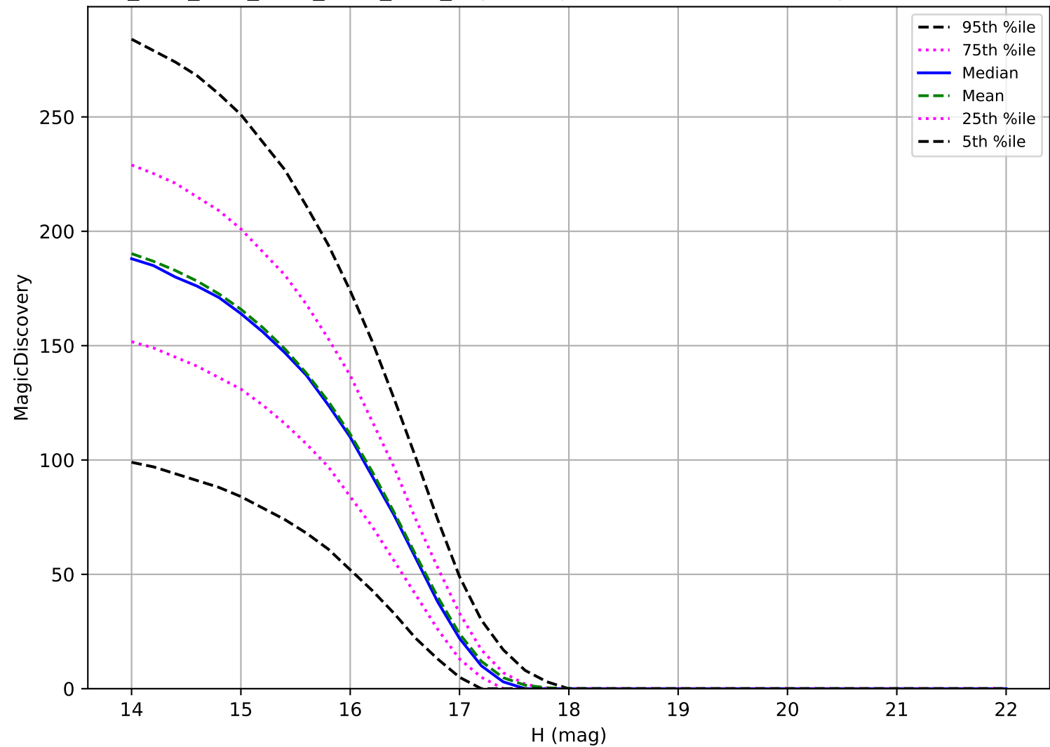
ddf_acor_sf15_lsf20_lsr50_v3.4_10yrs: Trojan 6 detections in 60 nights detection loss
