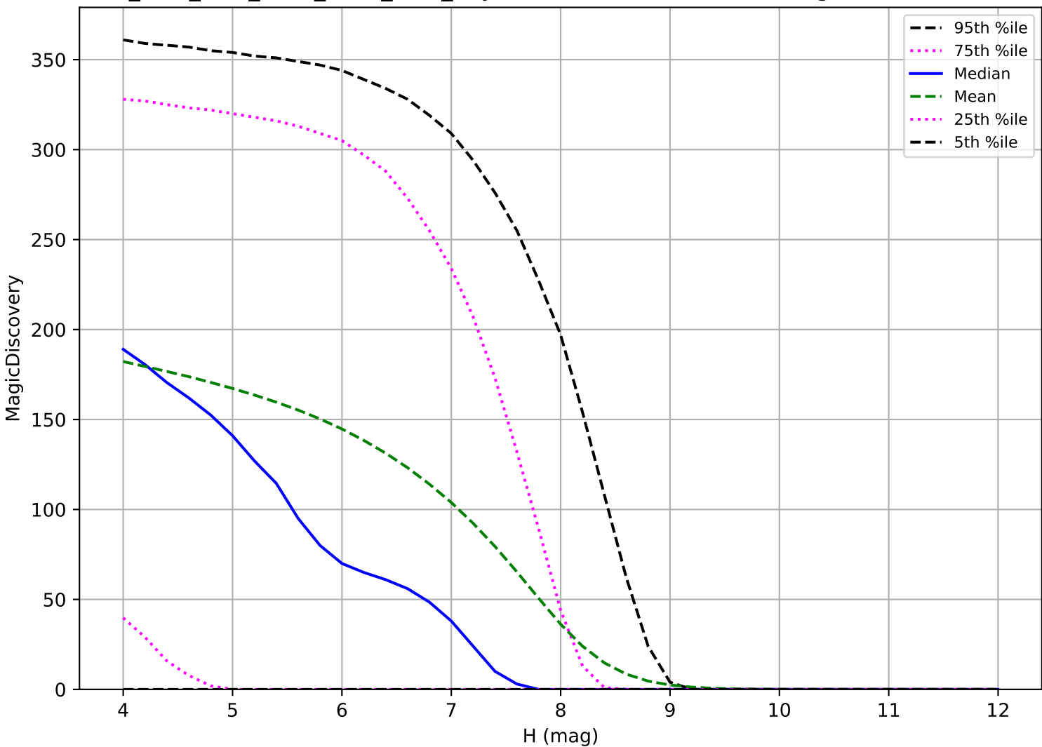
ddf_acor_sf15_lsf20_lsr50_v3.4_10yrs: TNO 6 detections in 60 nights detection loss
