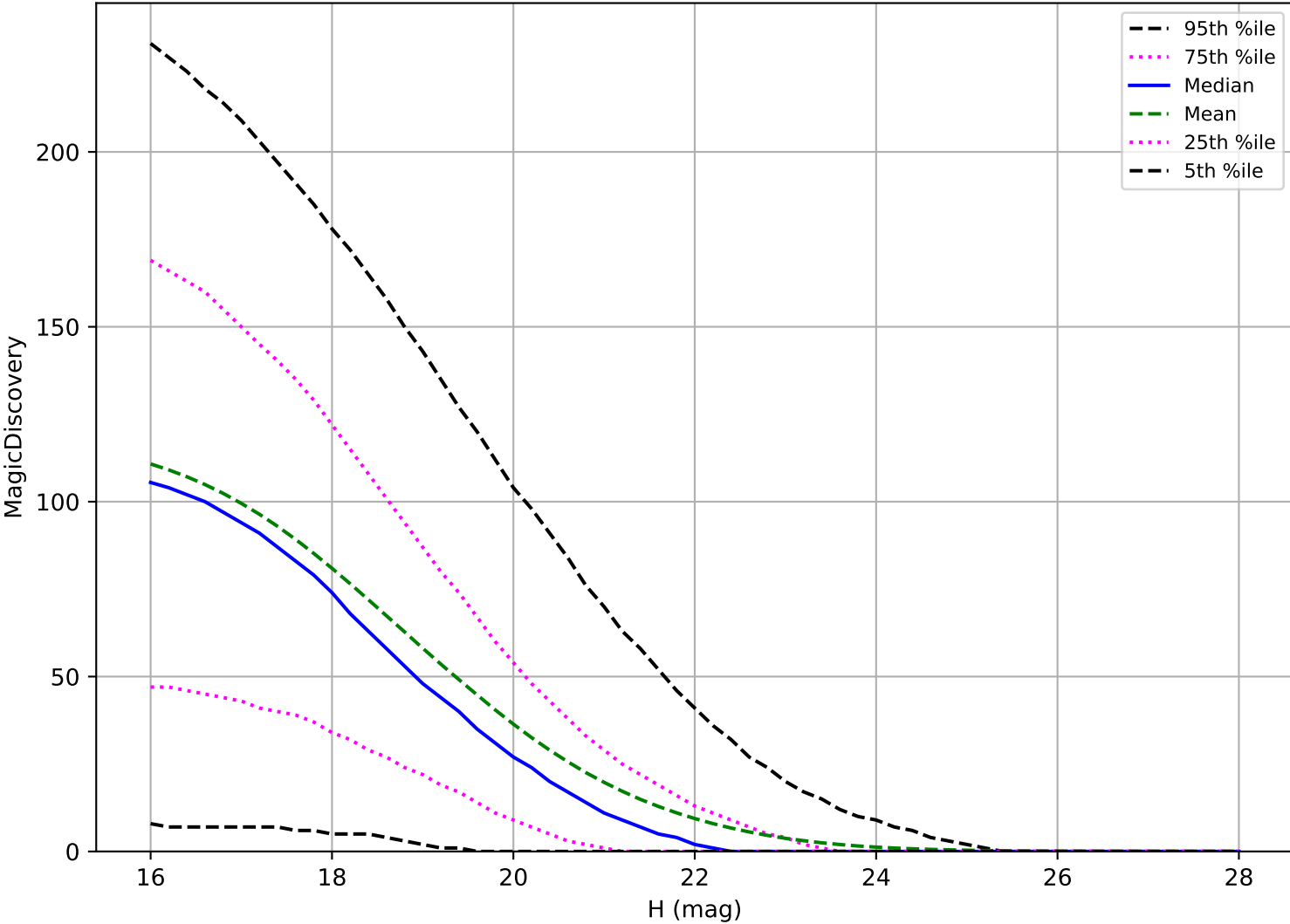
ddf_acor_sf15_lsf20_lsr50_v3.4_10yrs: PHA 6 detections in 60 nights detection loss
