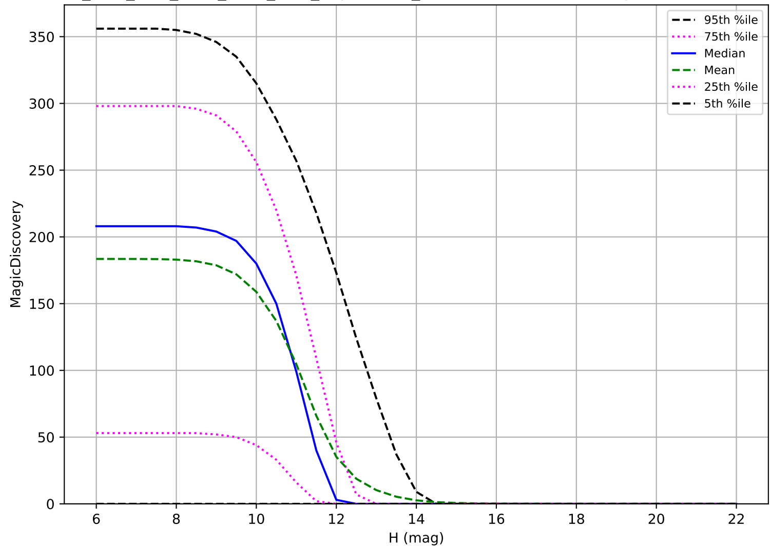
ddf_acor_sf15_lsf20_lsr50_v3.4_10yrs: OCC_r20 6 detections in 60 nights detection loss
