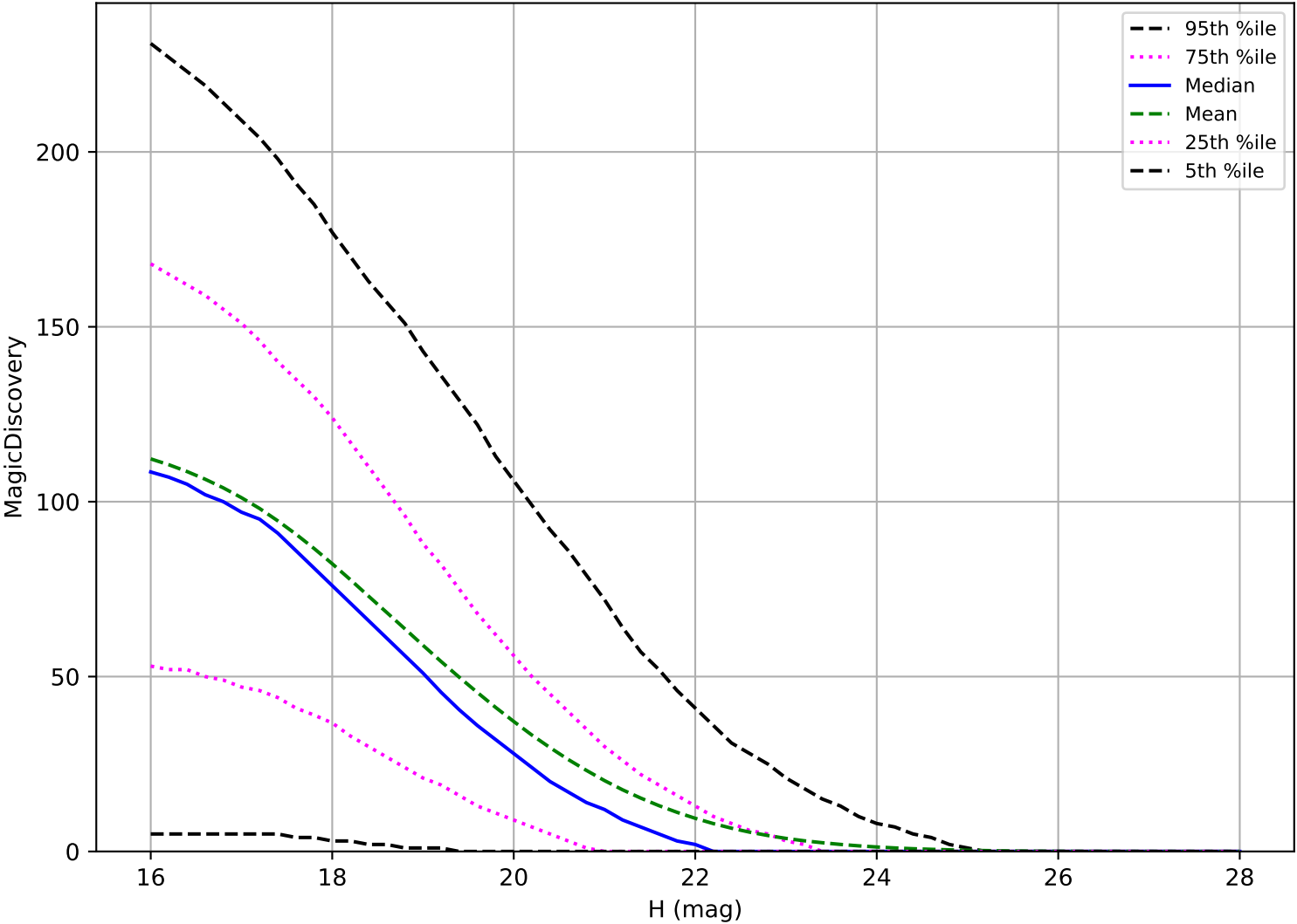
ddf_acor_sf15_lsf20_lsr50_v3.4_10yrs: NEO 6 detections in 60 nights detection loss
