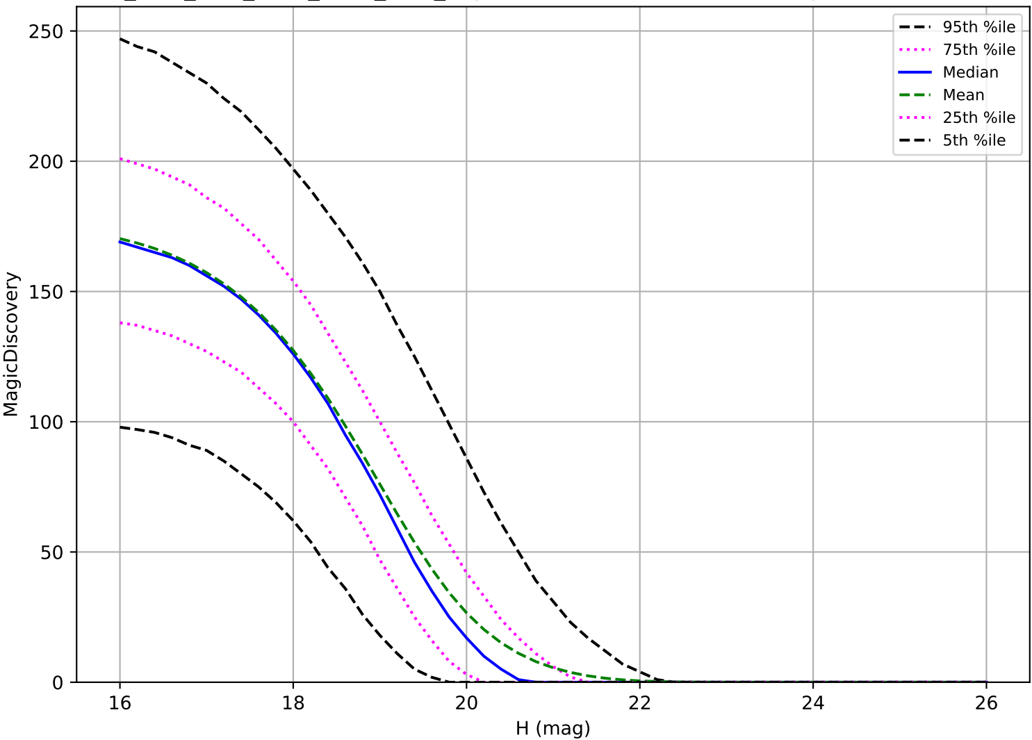
ddf_acor_sf15_lsf20_lsr50_v3.4_10yrs: MBA 6 detections in 60 nights detection loss
