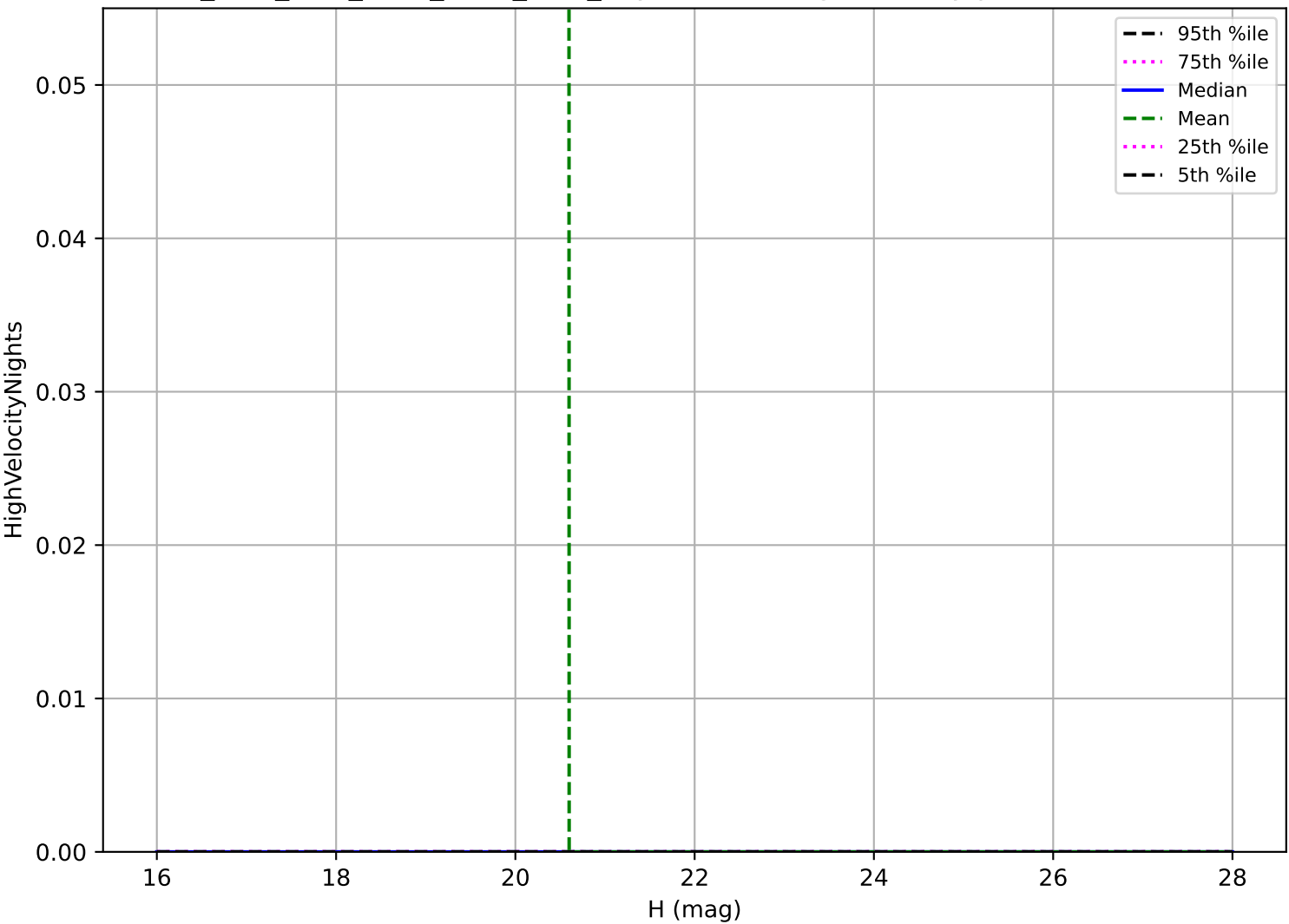
ddf_acor_sf15_lsf20_lsr50_v3.4_10yrs: Vatira High velocity pair detection loss
