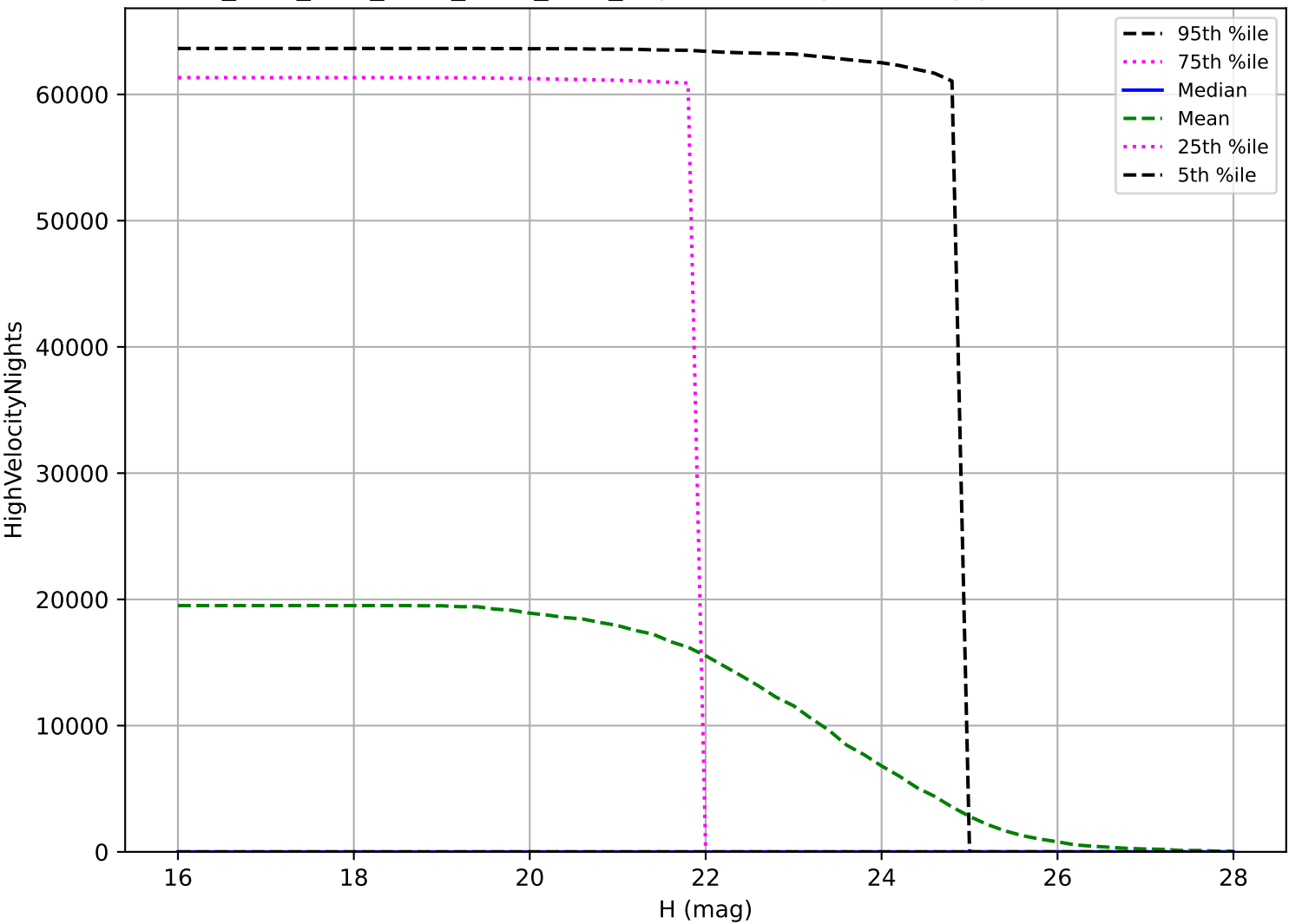
ddf_acor_sf15_lsf20_lsr50_v3.4_10yrs: NEO High velocity pair detection loss
