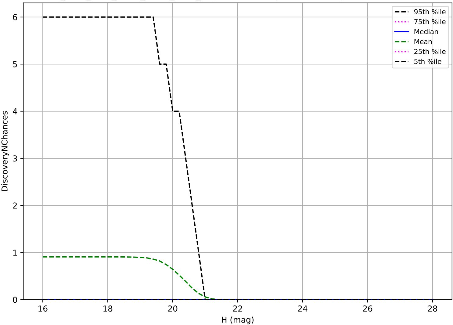
ddf_acor_sf15_lsf20_lsr50_v3.4_10yrs: Vatira 3 pairs in 15 nights detection loss
