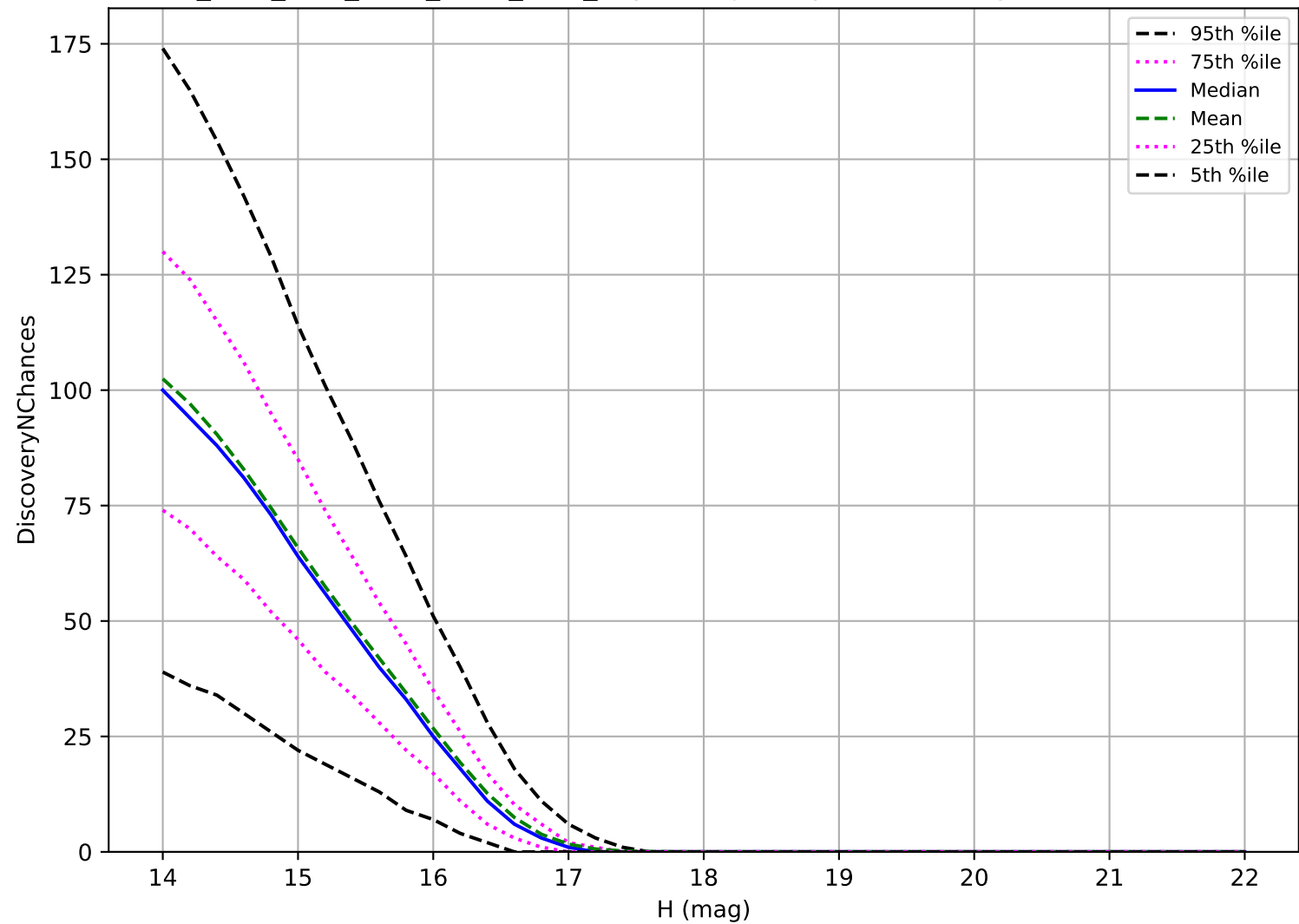
ddf_acor_sf15_lsf20_lsr50_v3.4_10yrs: Trojan 3 pairs in 15 nights detection loss
