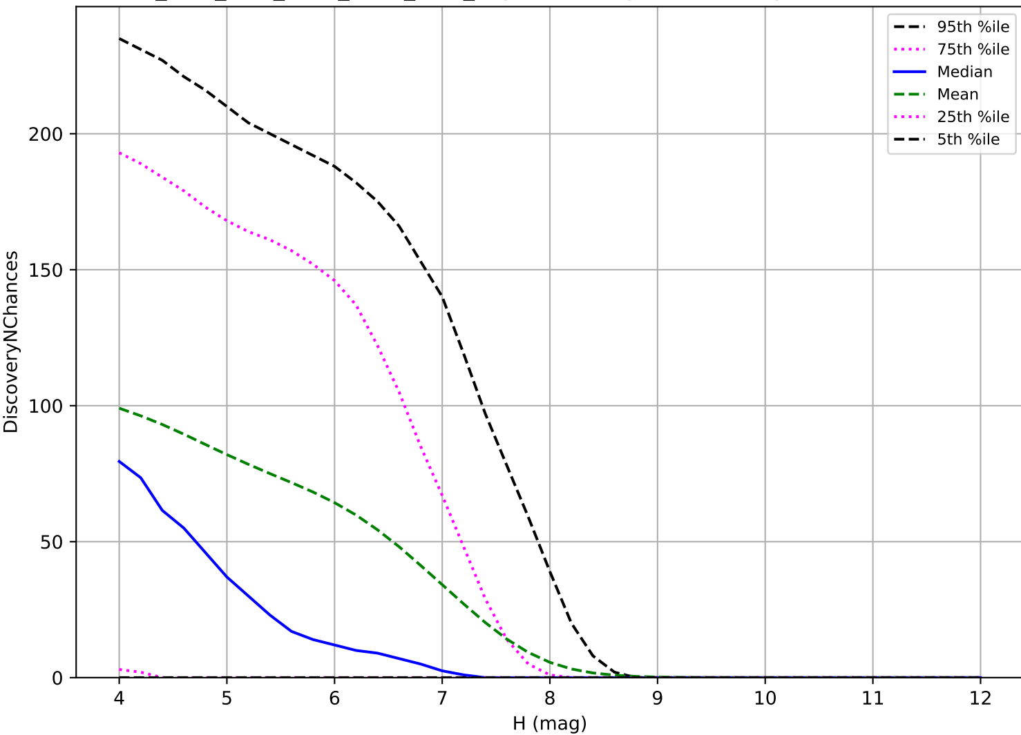
ddf_acor_sf15_lsf20_lsr50_v3.4_10yrs: TNO 3 pairs in 15 nights detection loss
