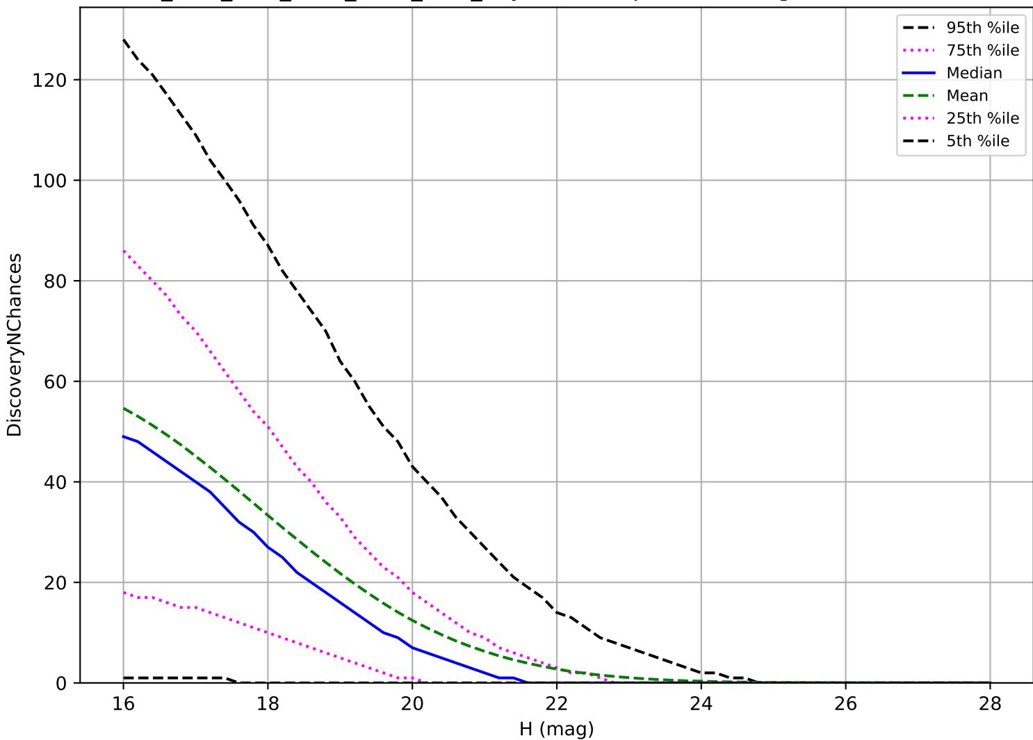
ddf_acor_sf15_lsf20_lsr50_v3.4_10yrs: PHA 3 pairs in 15 nights detection loss
