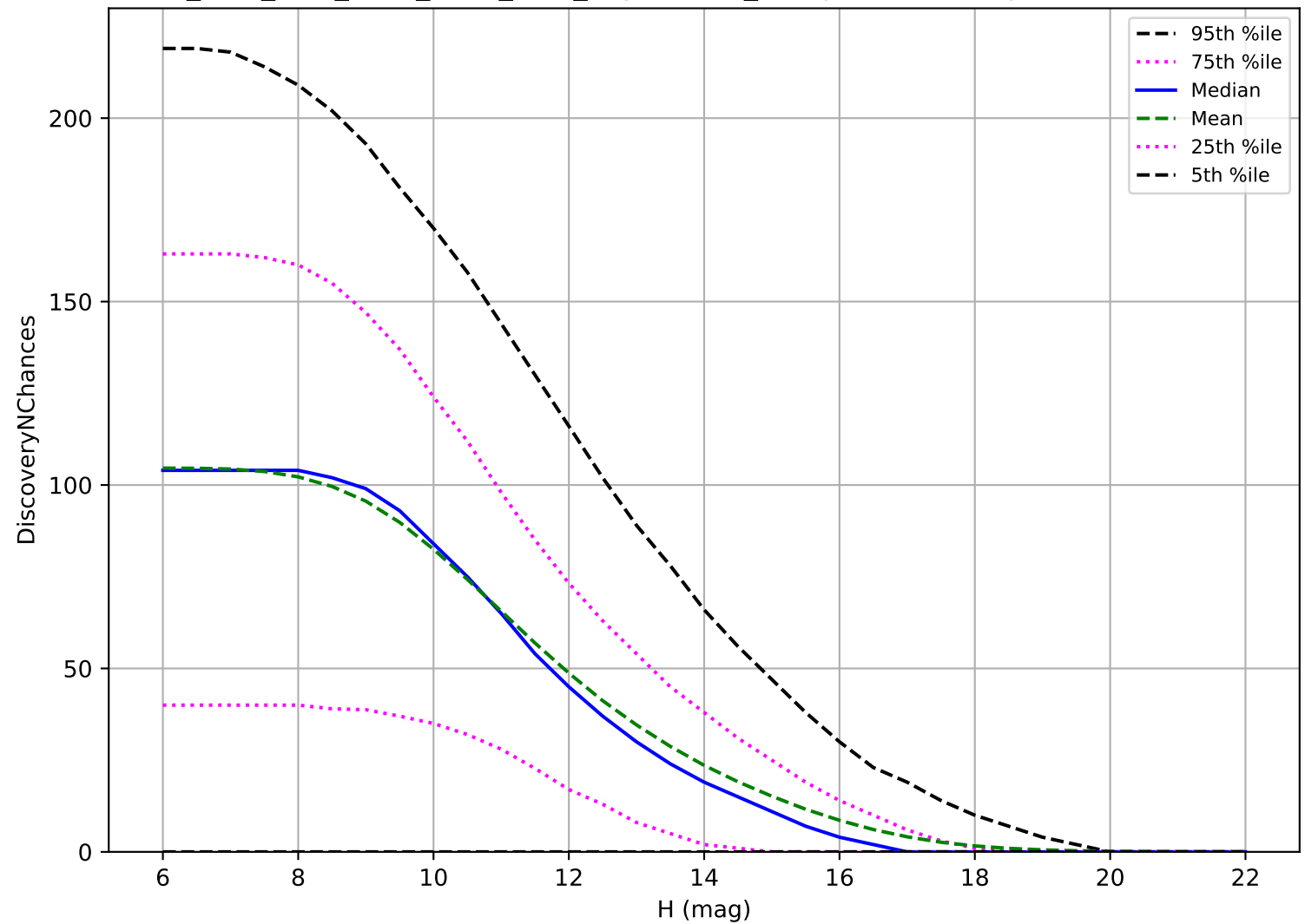
ddf_acor_sf15_lsf20_lsr50_v3.4_10yrs: OCC_r5 3 pairs in 15 nights detection loss
