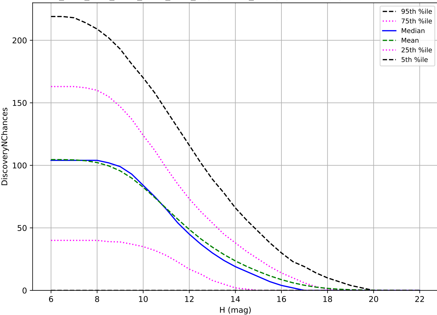
ddf_acor_sf15_lsf20_lsr50_v3.4_10yrs: OCC_r5 3 pairs in 15 nights detection loss
