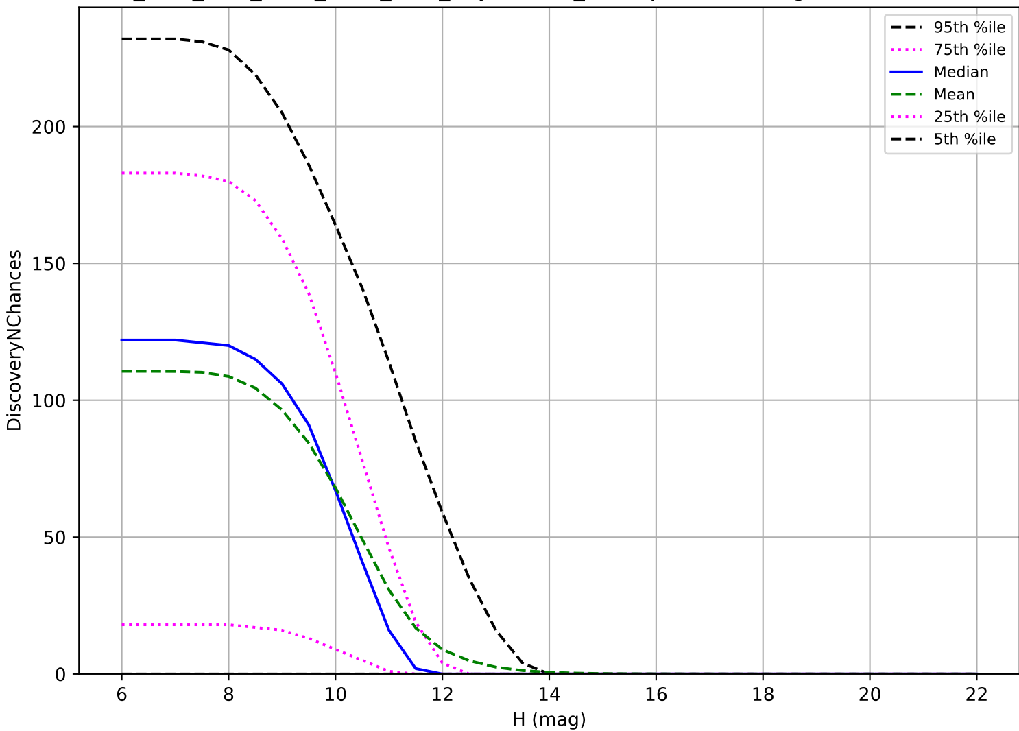
ddf_acor_sf15_lsf20_lsr50_v3.4_10yrs: OCC_r20 3 pairs in 15 nights detection loss
