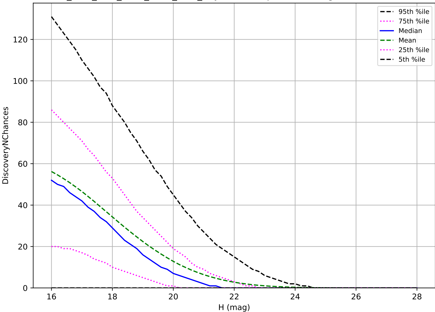
ddf_acor_sf15_lsf20_lsr50_v3.4_10yrs: NEO 3 pairs in 15 nights detection loss
