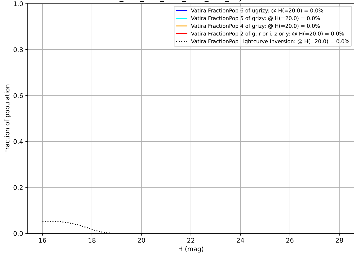
ddf_acor_sf15_lsf20_lsr50_v3.4_10yrs Vatira
