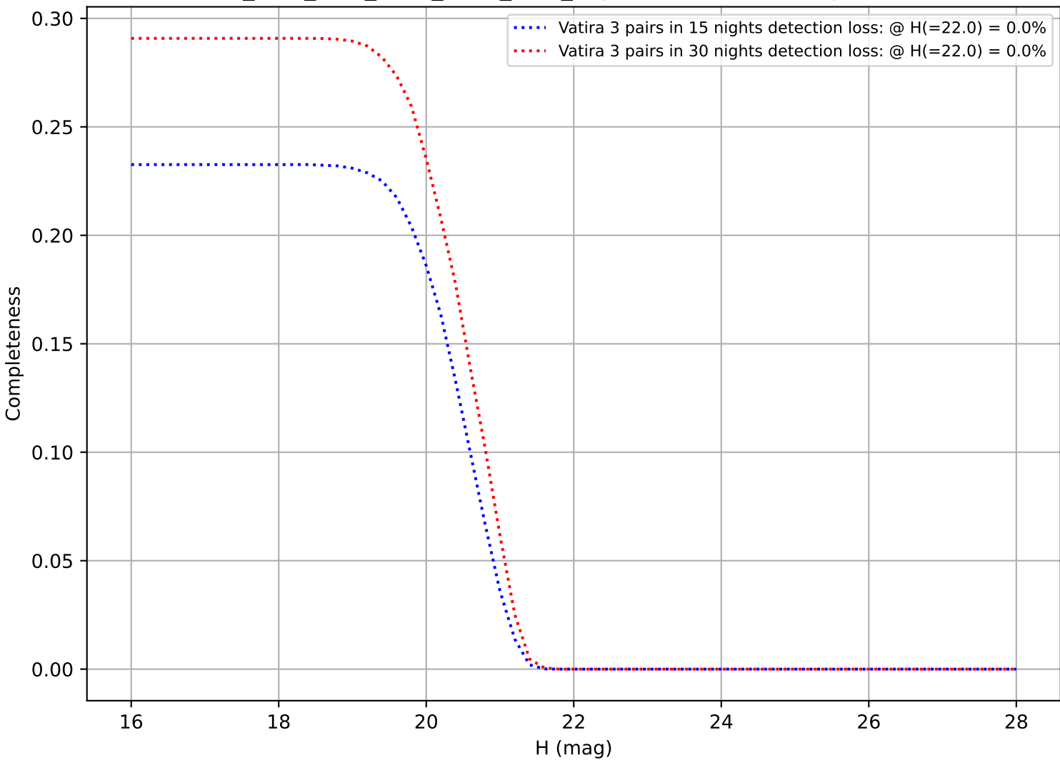
ddf_acor_sf15_lsf20_lsr50_v3.4_10yrs: DifferentialCompleteness
