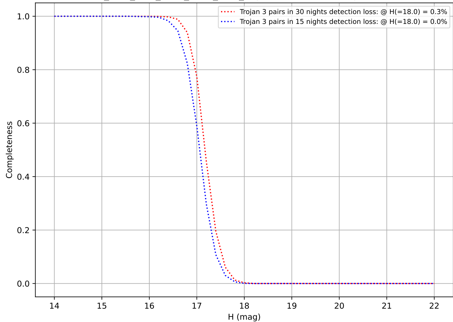
ddf_acor_sf15_lsf20_lsr50_v3.4_10yrs: DifferentialCompleteness
