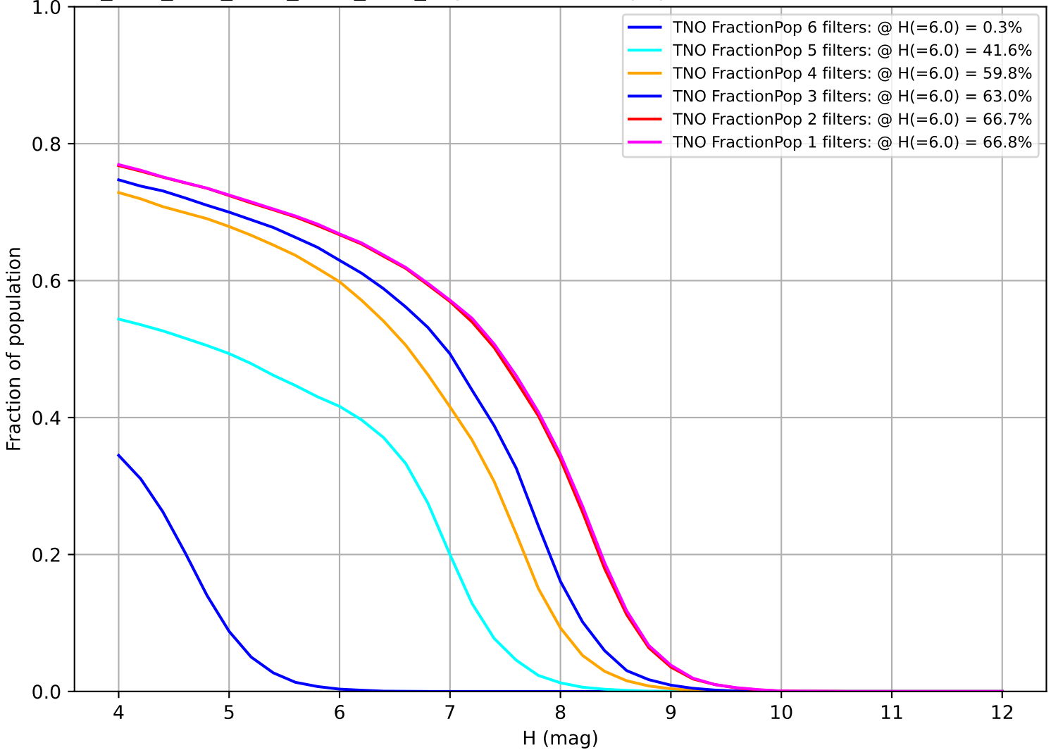
ddf_acor_sf15_lsf20_lsr50_v3.4_10yrs: Fraction of population with colors in X filters TNO
